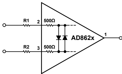
Figure 54. Input Protection
