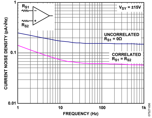
Figure 46. Current Noise Density vs. Frequency
